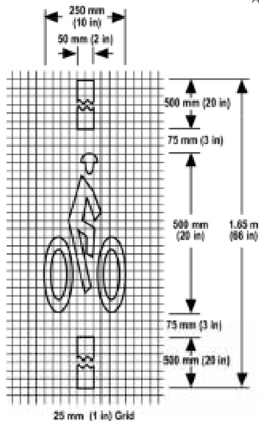
Figure 9C-7 – CA MUTCD
