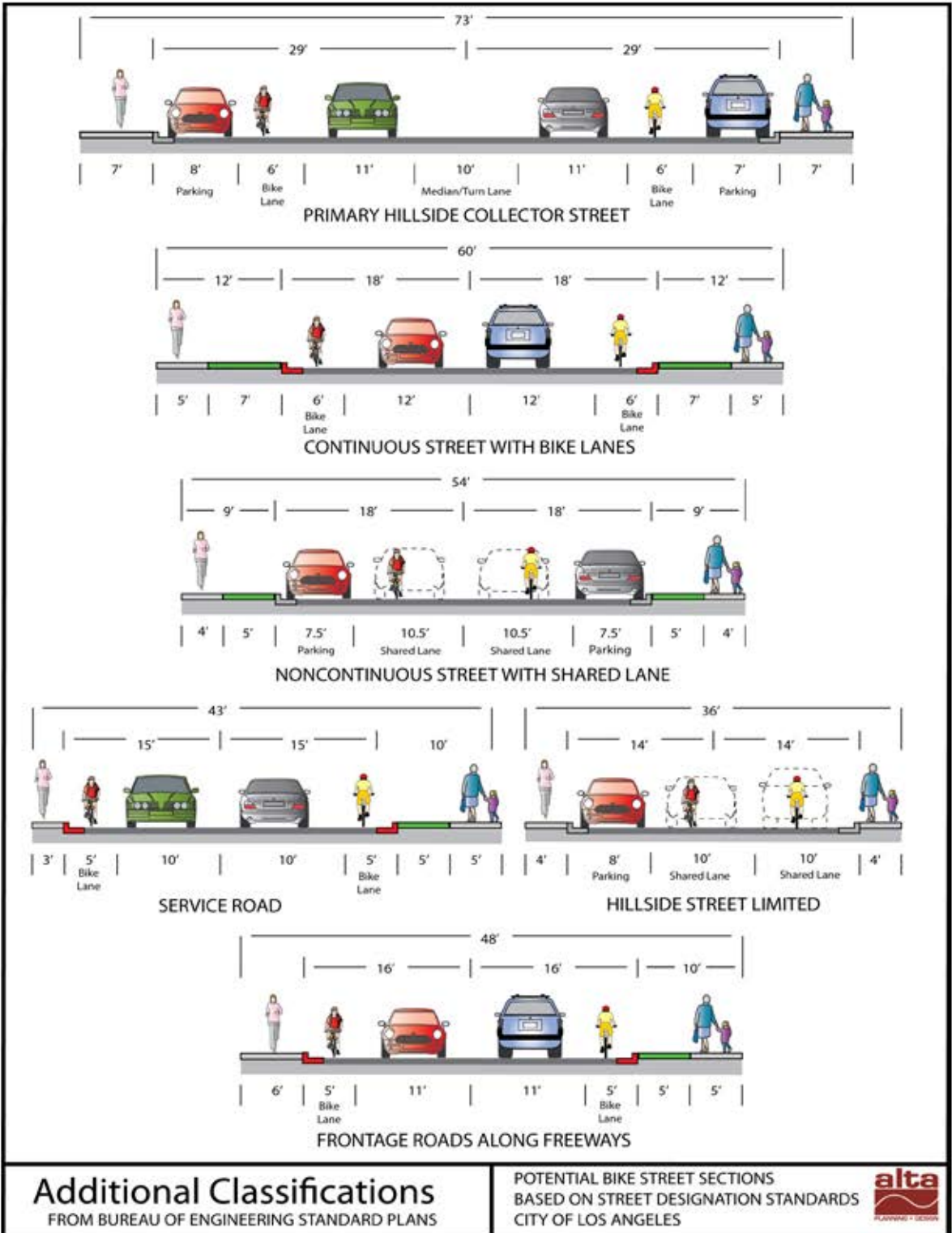
Figure 5-10. Additional Classifications - Complete Streets
