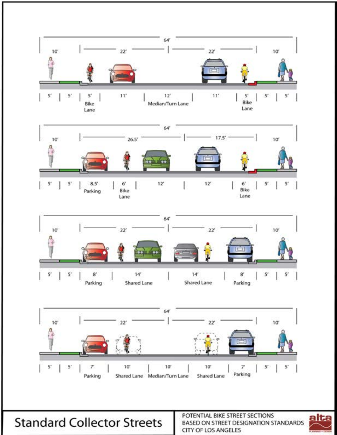
Figure 5-7. Standard Collector Streets - Complete Streets
