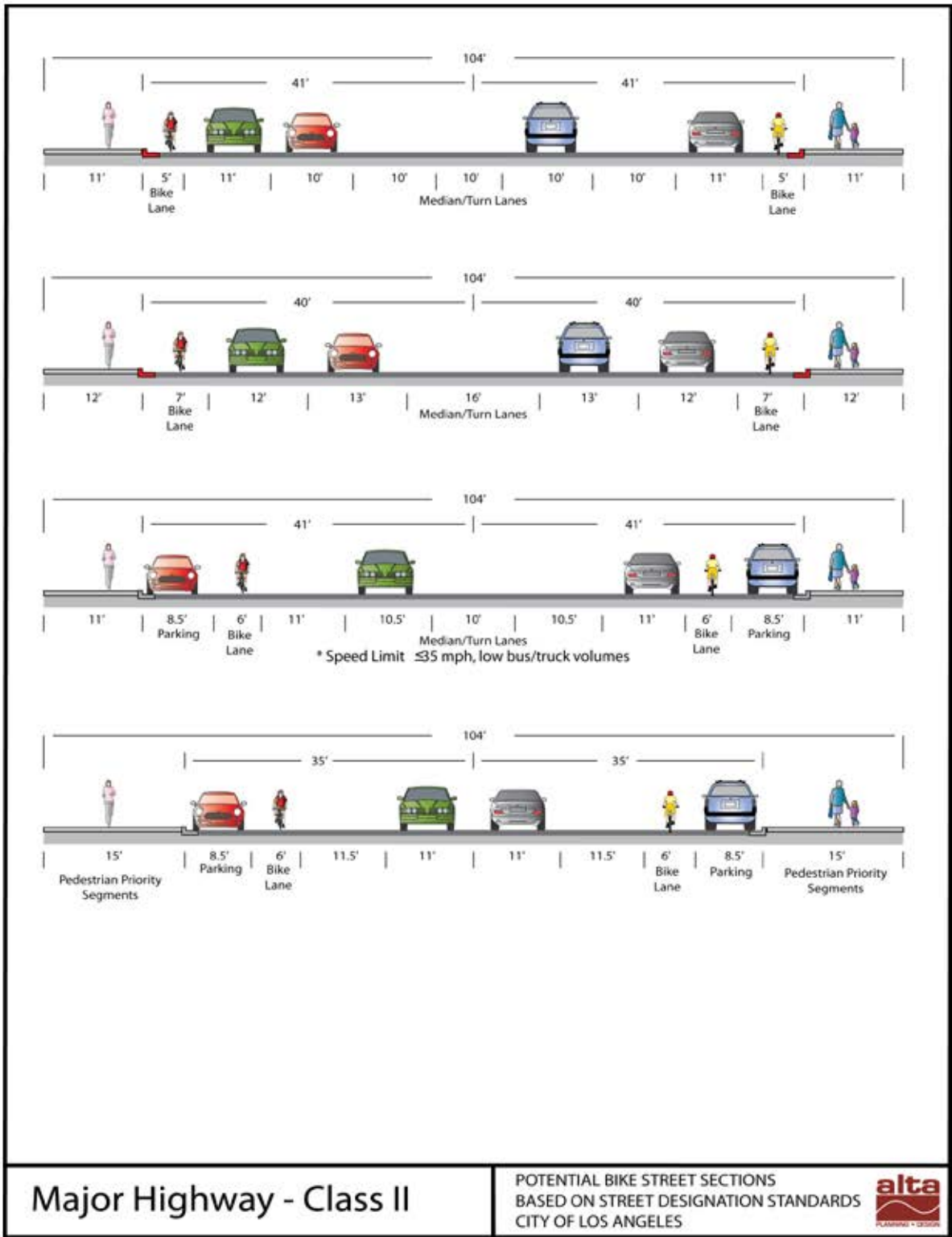
Figure 5-5. Major Highway - Class II - Complete Streets
