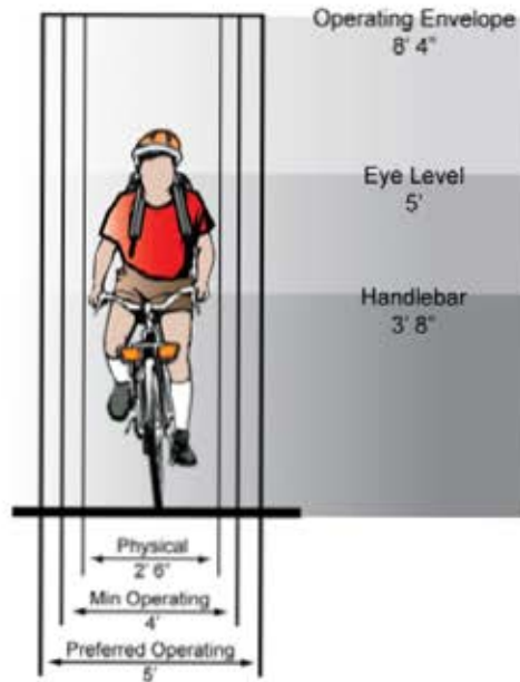
Figure 1-1. Standard Bicycle Rider Dimensions (AASHTO guide for development of bicycle facilities 1499)
