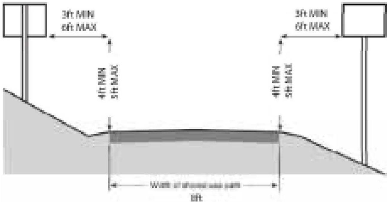
Figure 5 12 Signage Placement
