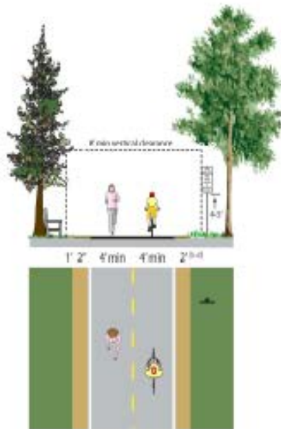
Class I Bicycle Path
