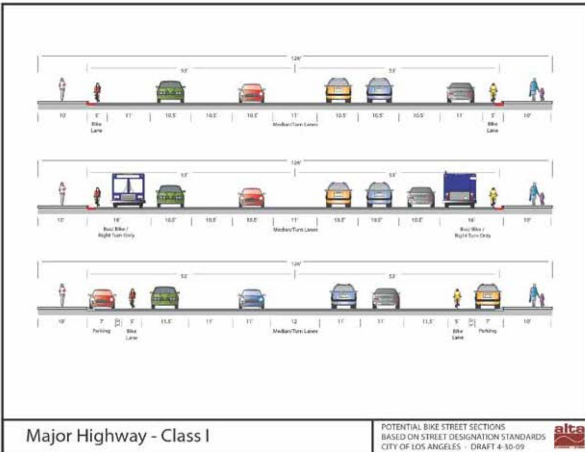
Figure 5-4. Major Highway - Class I - Complete Streets
