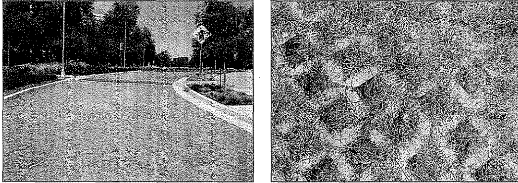
FIGURE 13. VEGETATED CONCRETE GRID PAVERS
