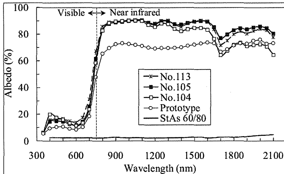
FIGURE 15. REFLECTIVITY WITH WAVELENGTH OF TRAIL PAINT COATINGS (KINOCHI, 2004).
