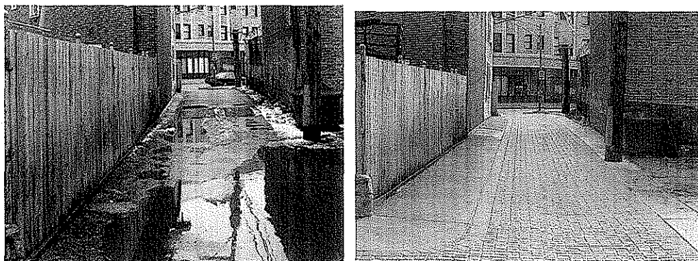
FIGURE 18. ALLEY WITH IMPERMEABLE PAVEMENT AND POOR DRAINAGE (LEFT) AND ALLEY INCORPORATING GREEN ALLEY PRINCIPLES (RIGHT) (CDOT).
