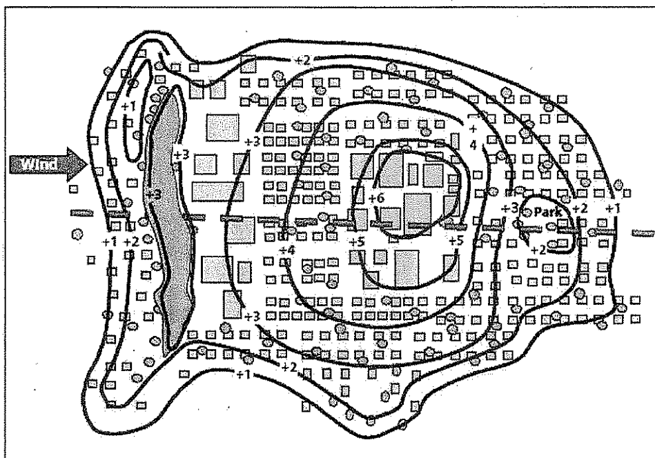
FIGURE 3. ISOTHERM MAP DEPICTING AN ATMOSPHERIC NIGHTTIME URBAN HEAT ISLAND (EPA, OCTOBER 2008).
