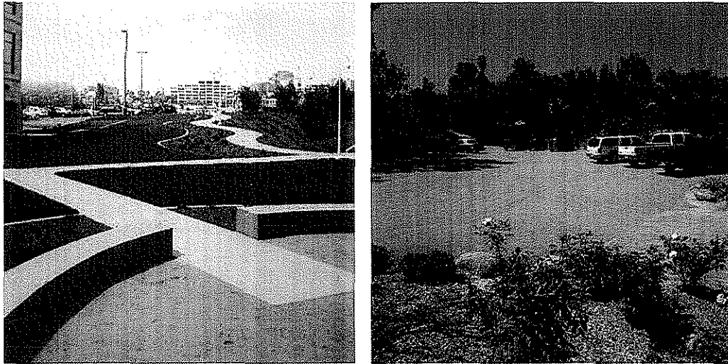
FIGURE 20. GRASSPAVE 2 FIRE LANE AND GRAVELPAVE 2 PARKING LOT (INVISIBLE STRUCTURES, INC.).
