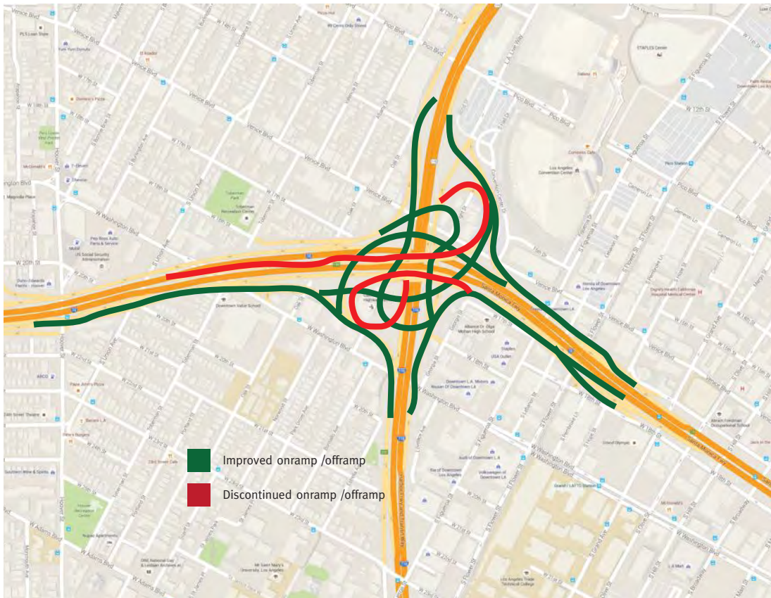
Figure 8: Interchange Design: I-10 and I-110
