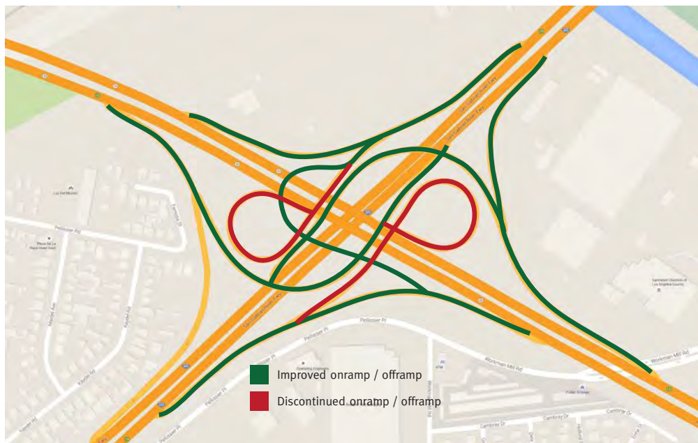
Figure 17: Interchange Design: I-605 and SR-60
