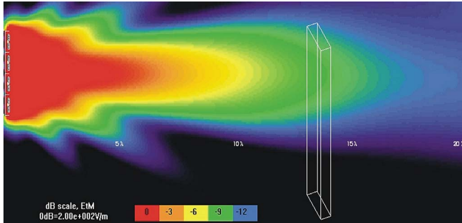
Figure 2. Electric field distribution radiated by the isolated 4 \times 1 antenna in the vertical plane containing the dipoles. Frequency: 1800 MHz; radiated power: 30 W.
