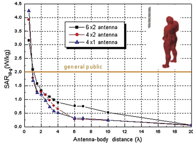
Figure 8. Maximum SAR_{10g} as a function of antenna–body distance. Frequency: 900 MHz; radiated power: 30 W.
