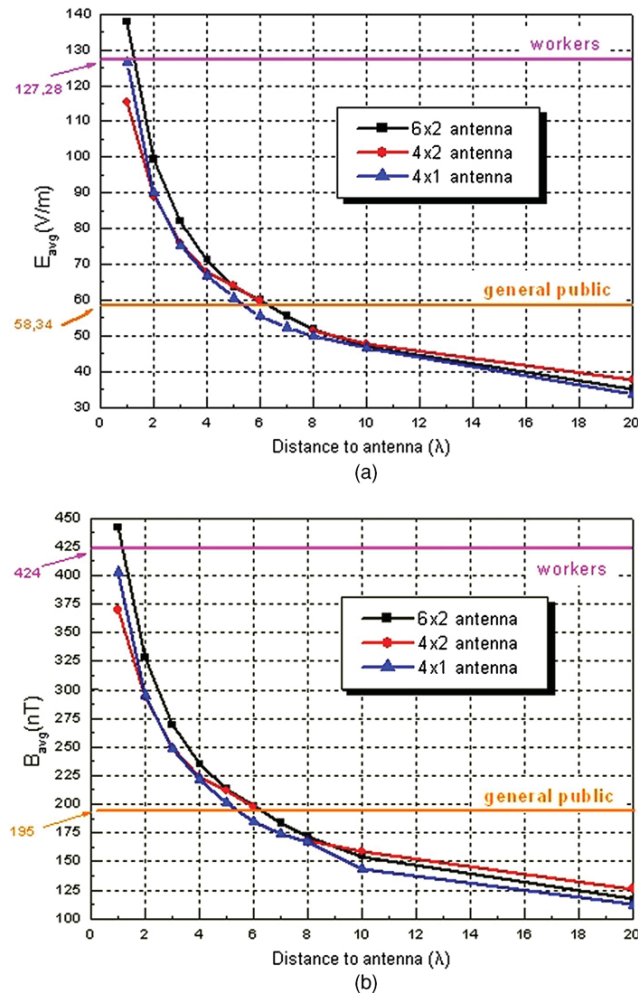
Figure 5. Averaged field strengths as a function of the distance to the antenna. Frequency: 1800 MHz; radiated power: 30 W. (a) Electric field intensity; (b) magnetic flux density.
