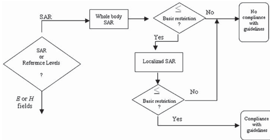
Figure 3. Methodology for guidelines compliance assessment via SAR.
