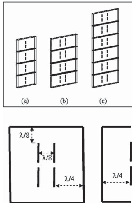
Figure 1. Geometry of antennas: (a) 4 \times 1 array; (b) 4 \times 2 array; (c) 6 \times 2 array.
