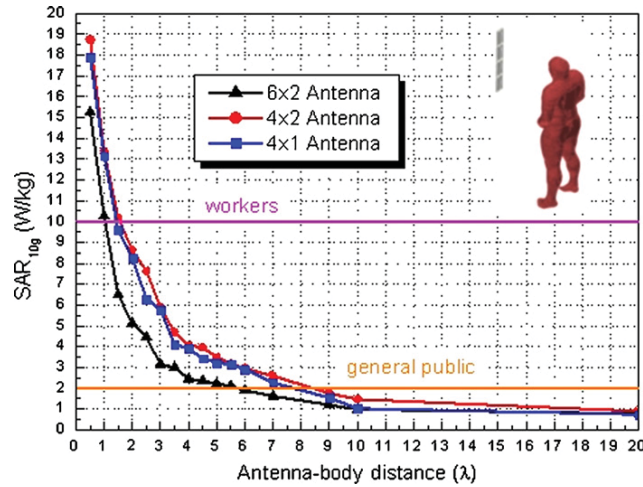
Figure 10. Maximum SAR 10g as a function of antenna–body distance. Frequency: 2170 MHz; radiated power: 30 W.
