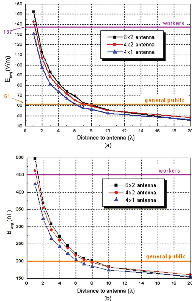
Figure 6. Averaged field strengths as a function of the distance to the antenna. Frequency: 2170 MHz; radiated power: 30 W. (a) Electric field intensity; (b) magnetic flux density.
