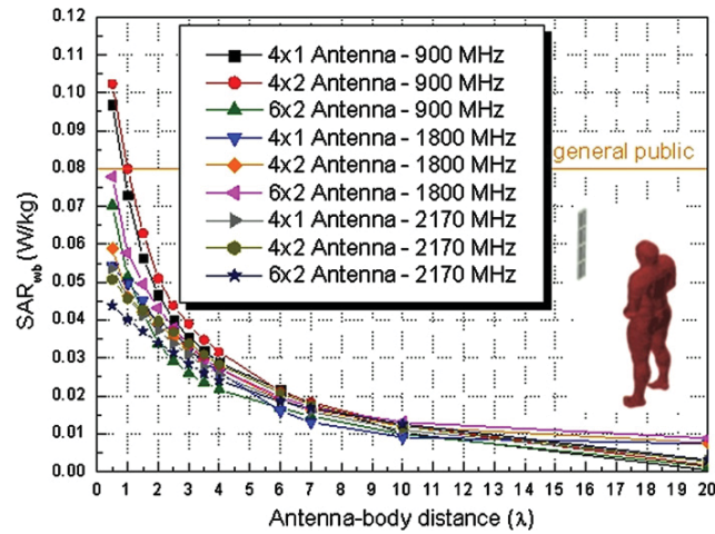
Figure 7. SAR_{wb} as a function of antenna–body distance for all considered frequencies. Radiated power: 30 W.
