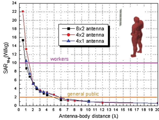
Figure 9. Maximum SAR 10g as a function of antenna–body distance. Frequency: 1800 MHz; radiated power: 30 W.
