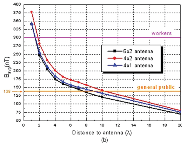
Figure 4. Averaged field strengths as a function of the distance to the antenna. Frequency: 900 MHz; radiated power: 30 W. (a) Electric field intensity; (b) magnetic flux density.
