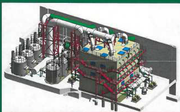
Wastewater Biotrickling Odor Control
